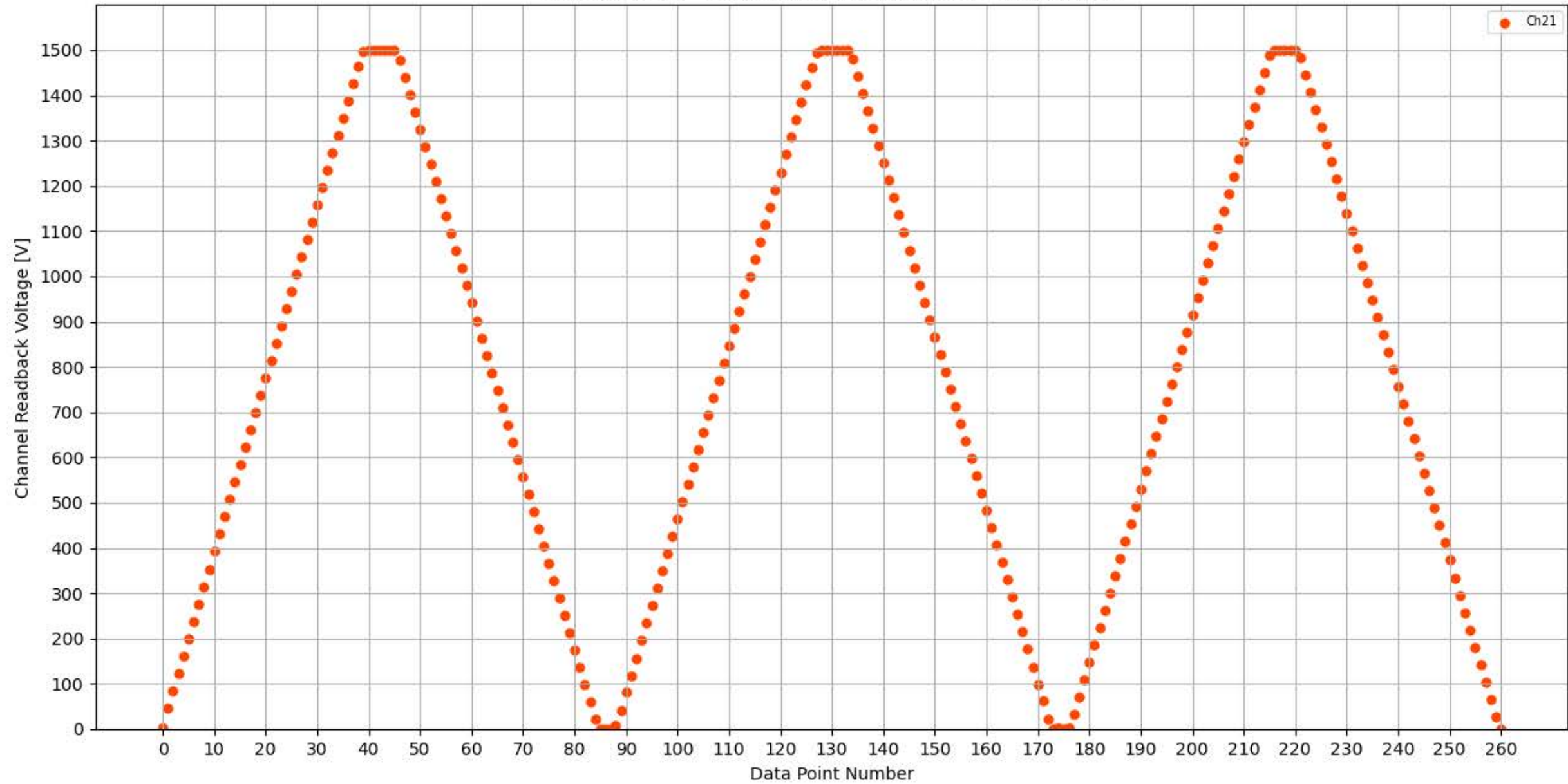
Voltage Ramp Test (Python) Bd #325, Slot #15, Ch #21
