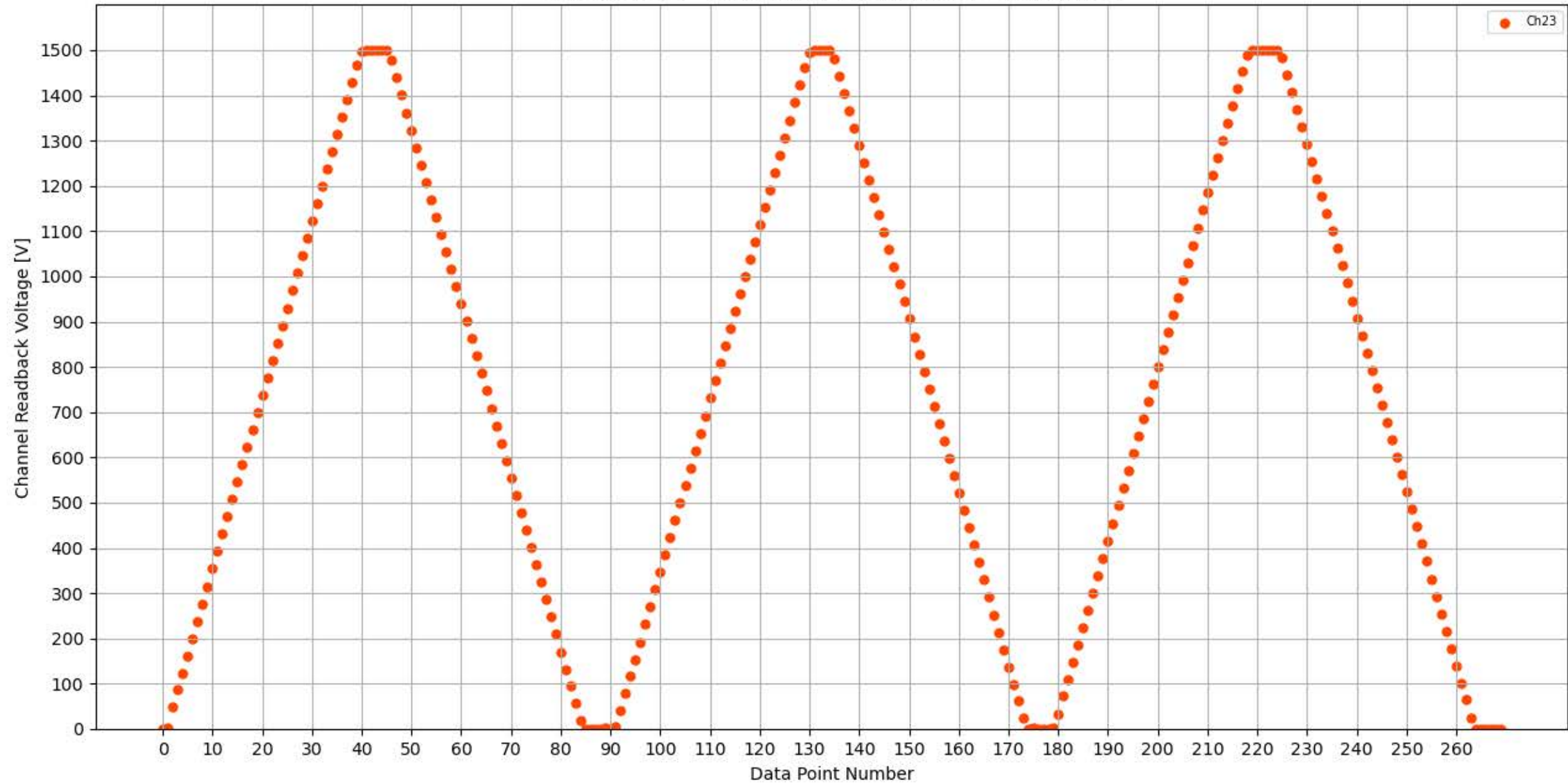
Voltage Ramp Test (Python) Bd #325, Slot #15, Ch #23
