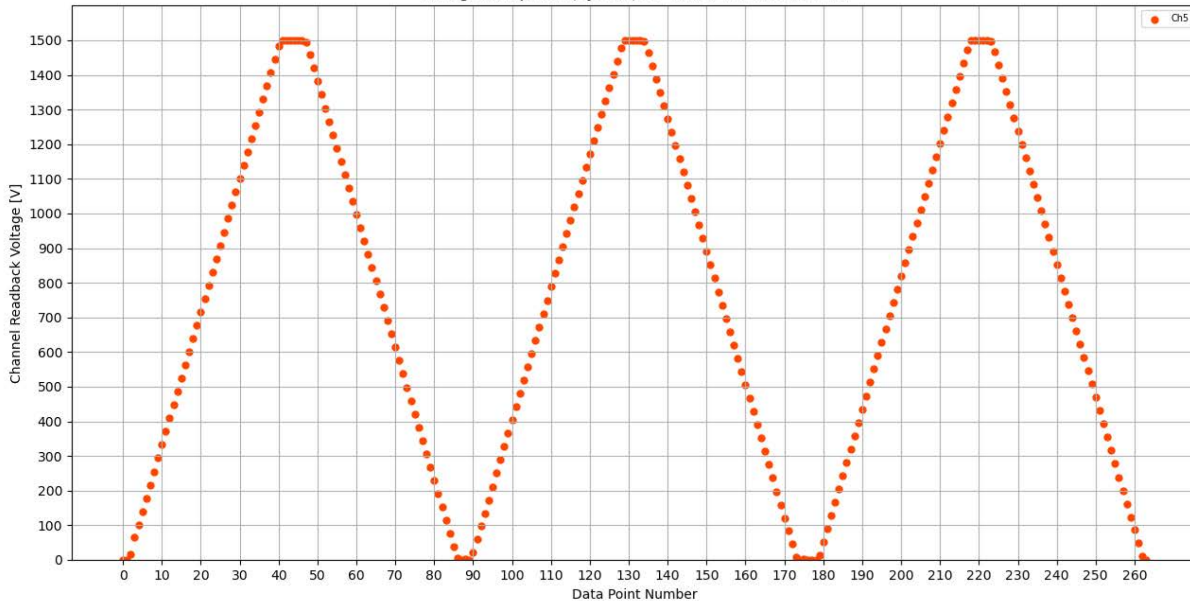
Voltage Ramp Test (Python) Bd #325, Slot #15, Ch #5
