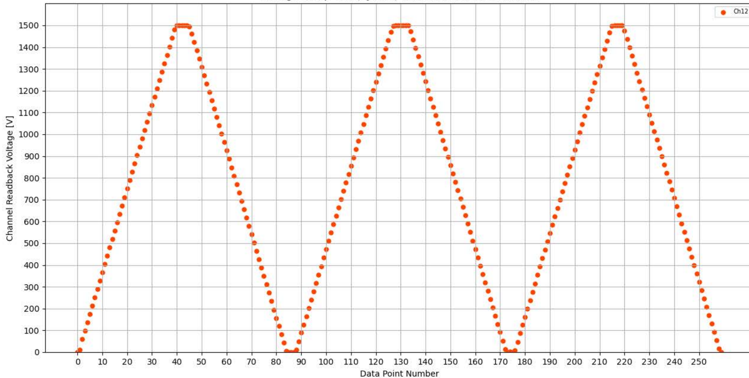
Voltage Ramp Test (Python) Bd #325, Slot #15, Ch #12
