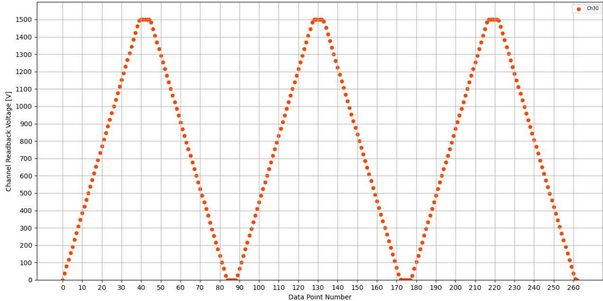
Voltage Ramp Test (Python) Bd #325, Slot #15, Ch #30
