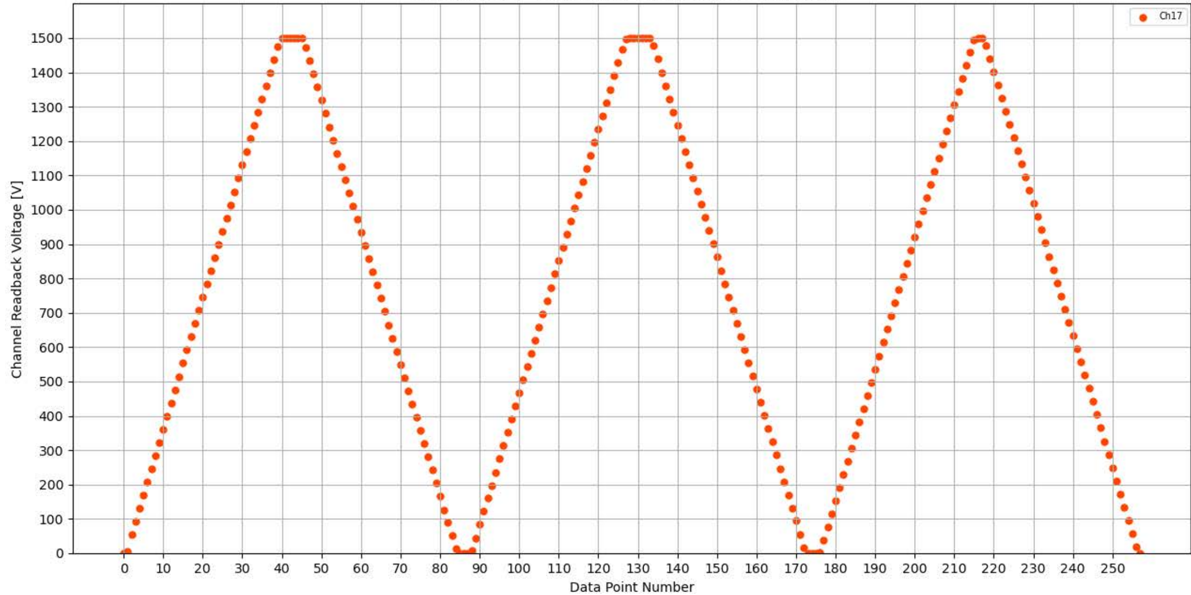
Voltage Ramp Test (Python) Bd #325, Slot #15, Ch #17
