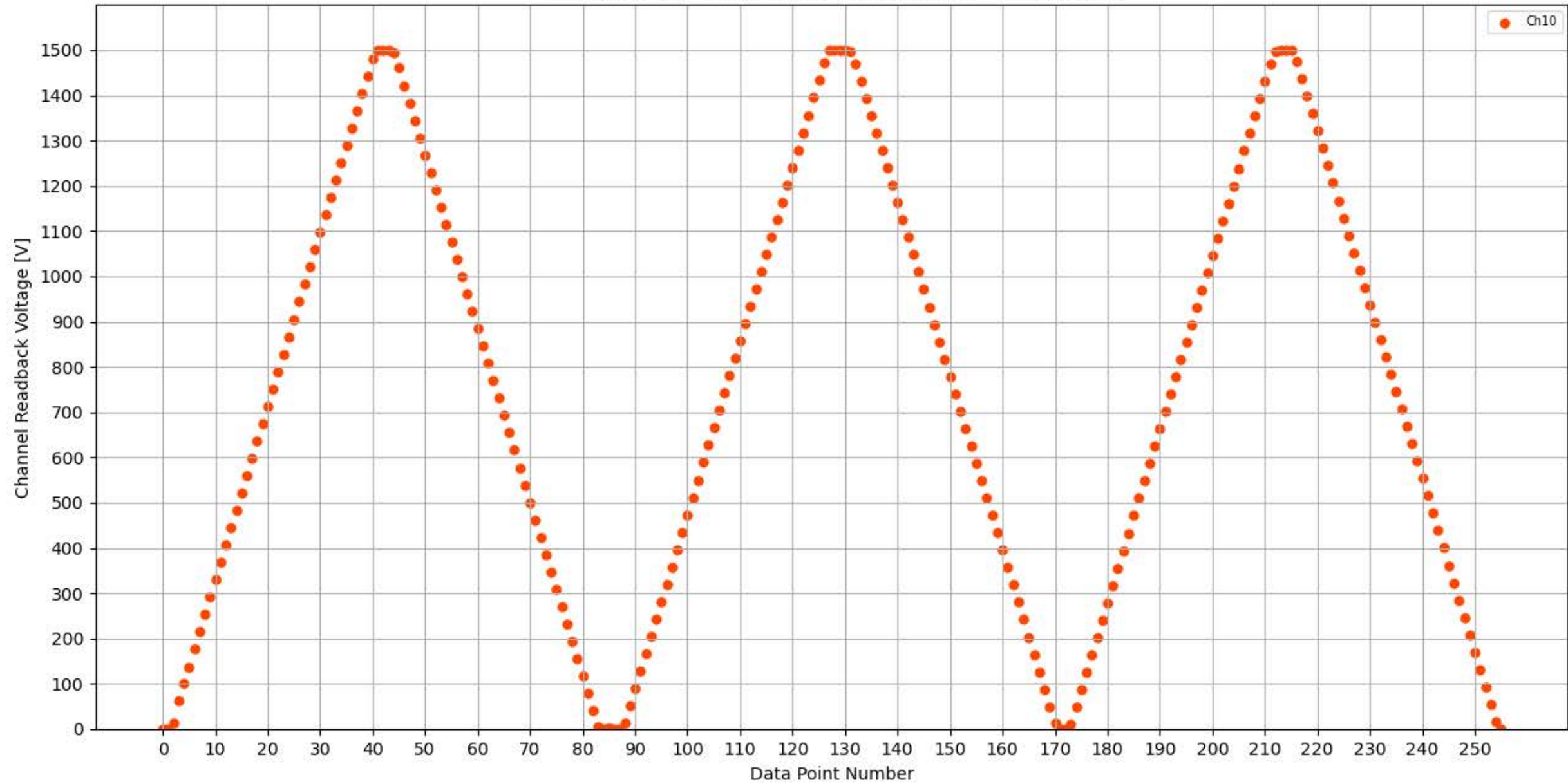
Voltage Ramp Test (Python) Bd #325, Slot #15, Ch #10
