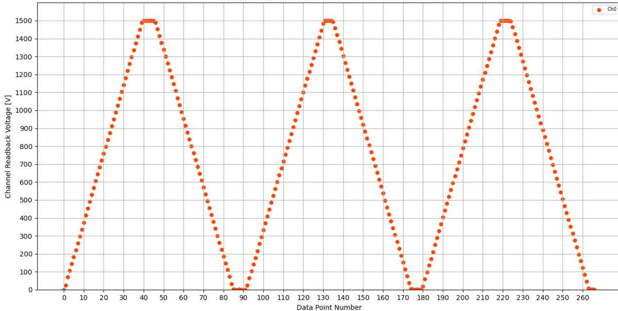
Voltage Ramp Test (Python) Bd #325, Slot #15, Ch #0
