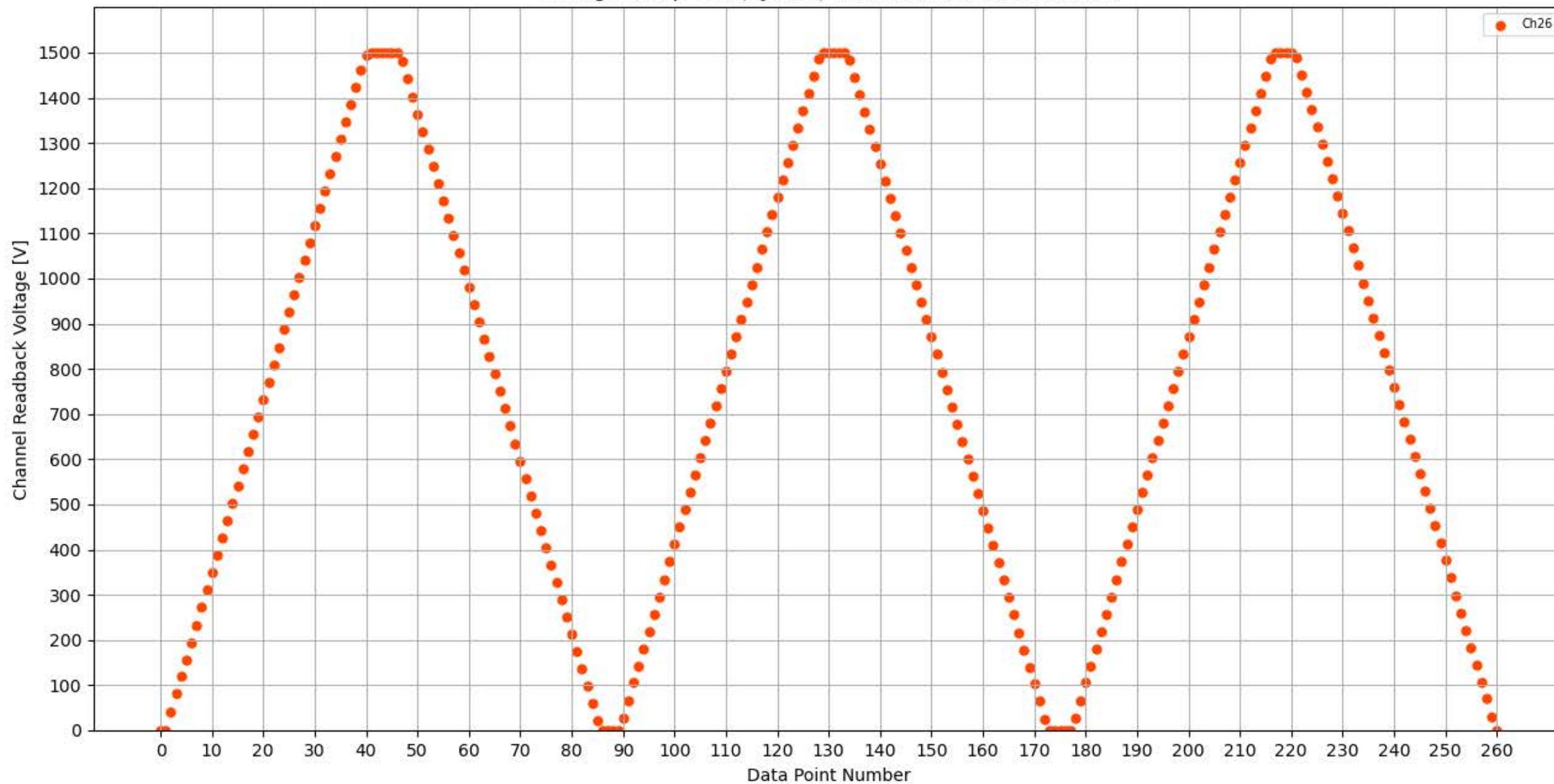
Voltage Ramp Test (Python) Bd #325, Slot #15, Ch #26
