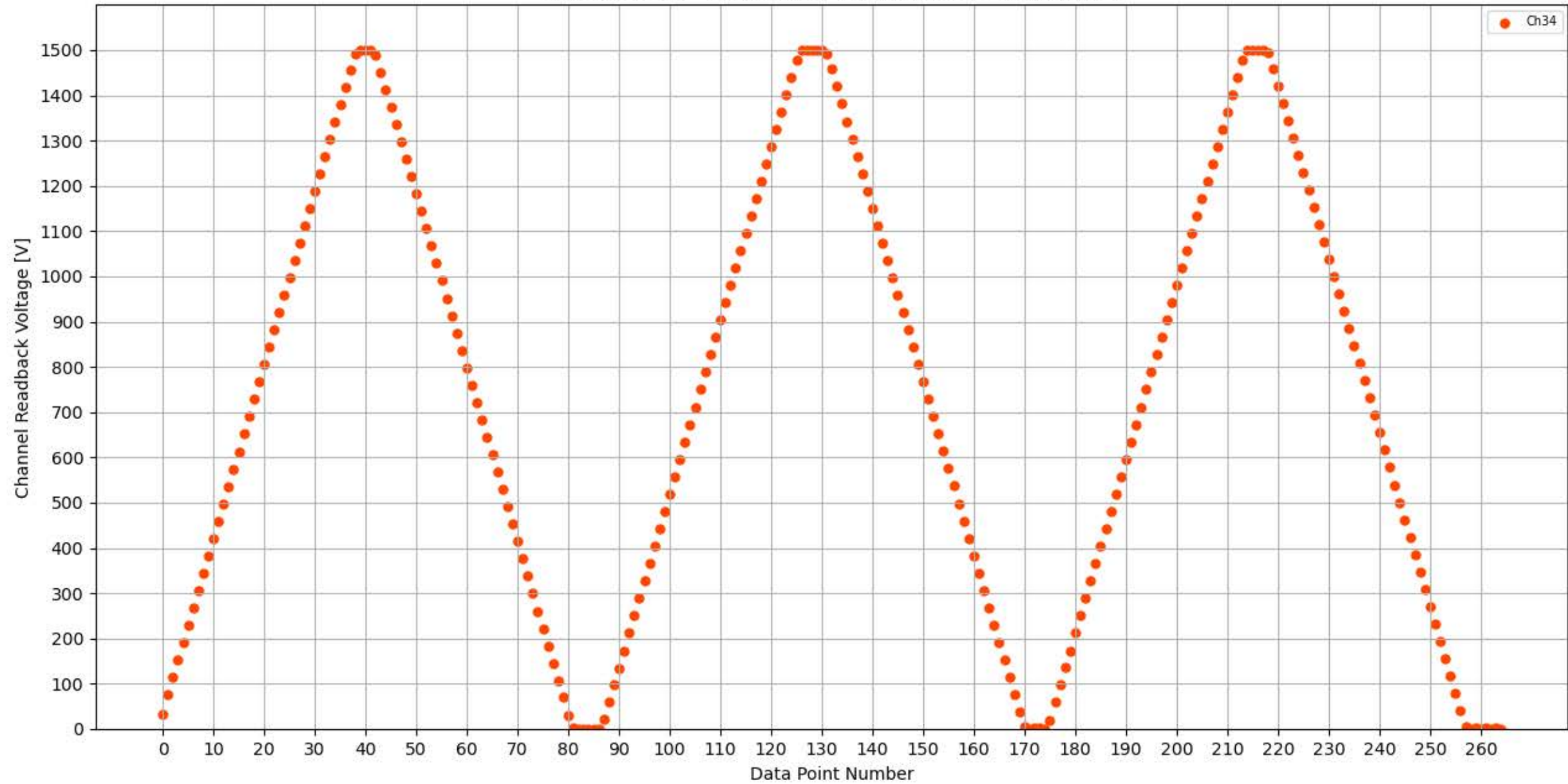
Voltage Ramp Test (Python) Bd #325, Slot #15, Ch #34
