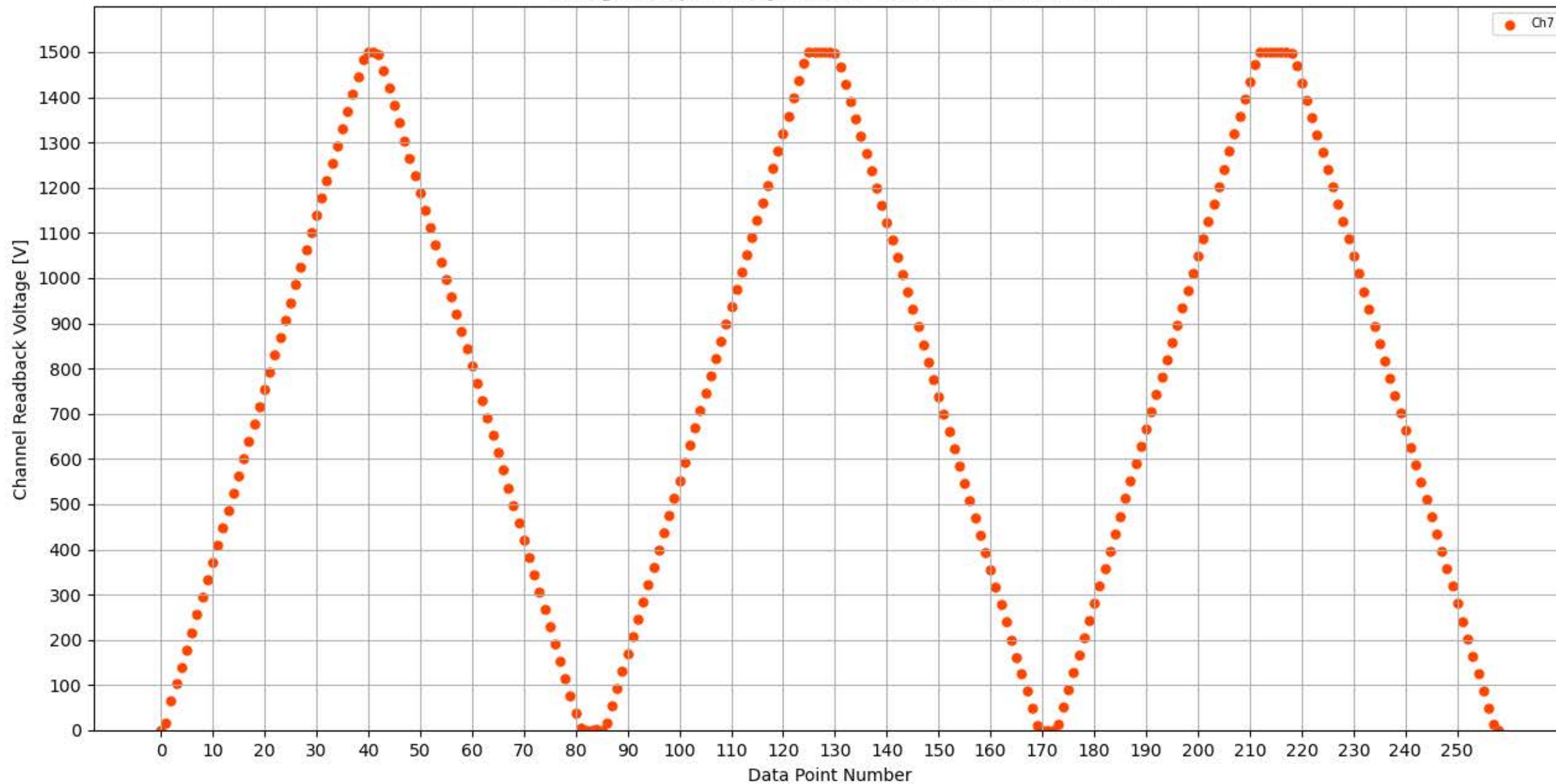
Voltage Ramp Test (Python) Bd #325, Slot #15, Ch #7
