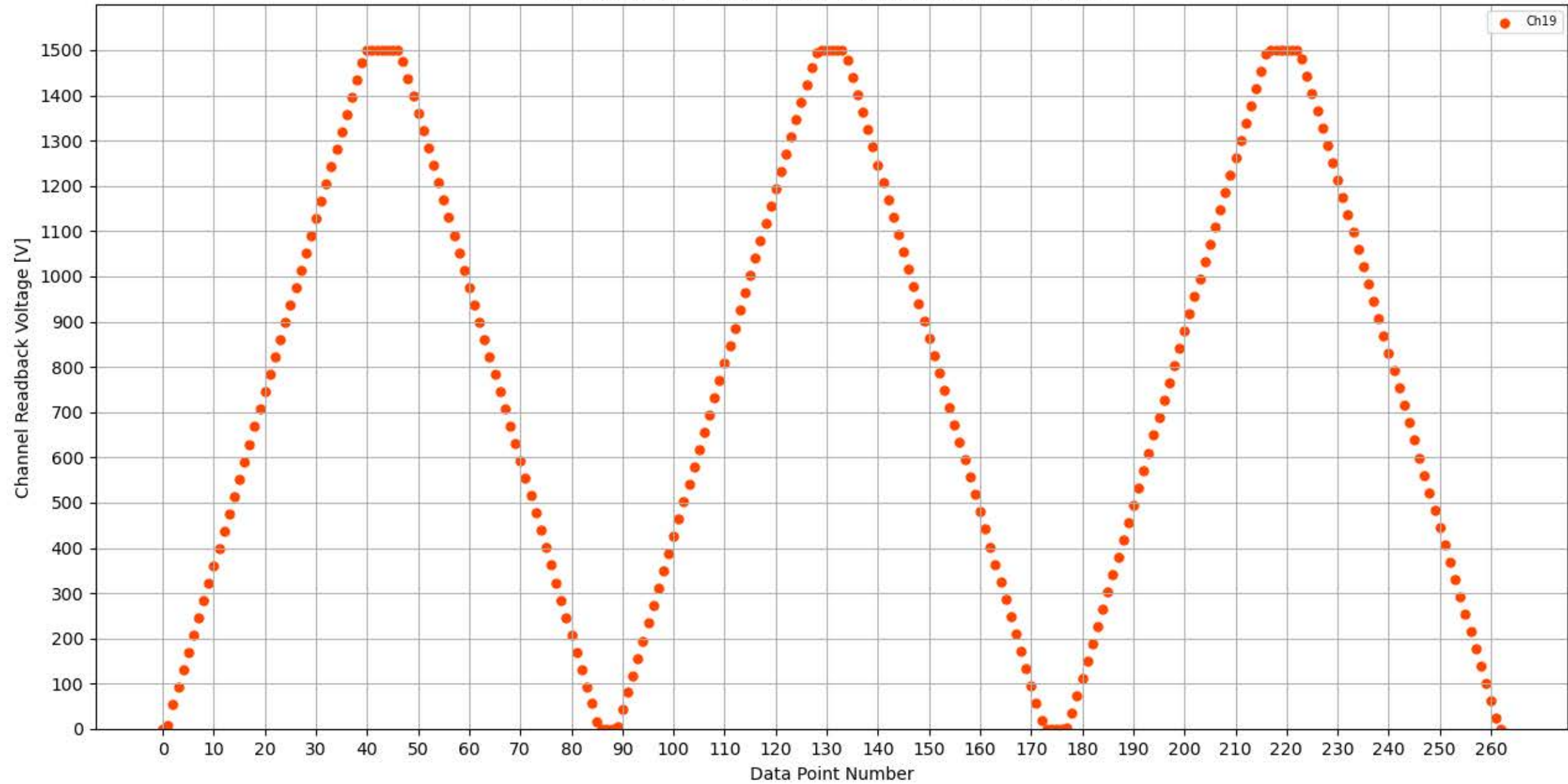
Voltage Ramp Test (Python) Bd #325, Slot #15, Ch #19
