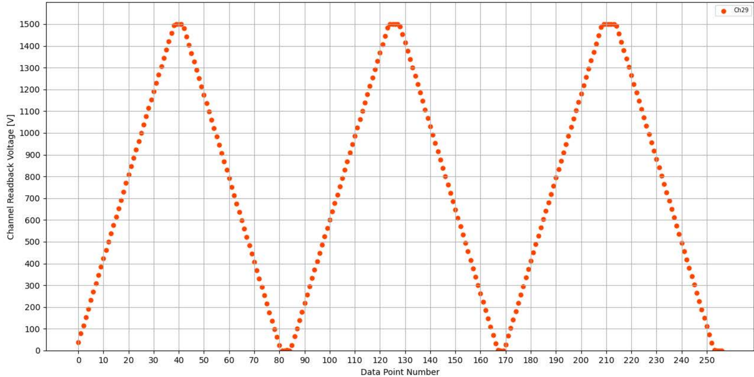
Voltage Ramp Test (Python) Bd #325, Slot #15, Ch #29
