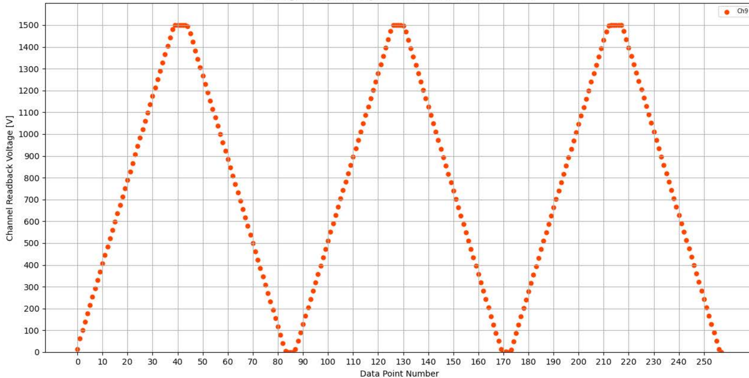
Voltage Ramp Test (Python) Bd #325, Slot #15, Ch #9
