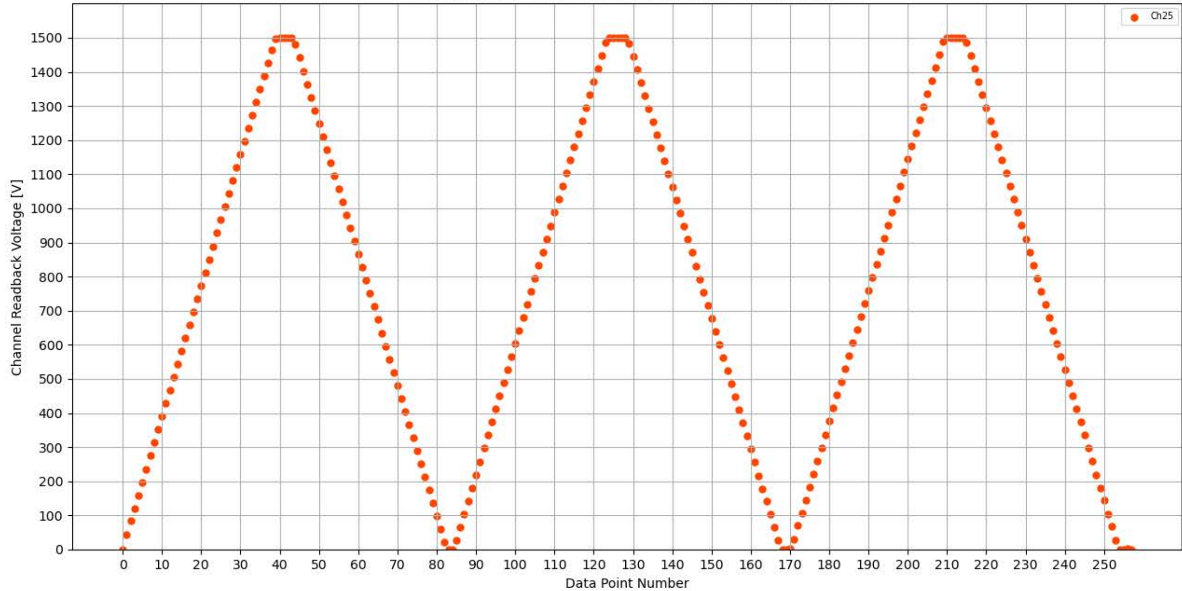
Voltage Ramp Test (Python) Bd #325, Slot #15, Ch #25
