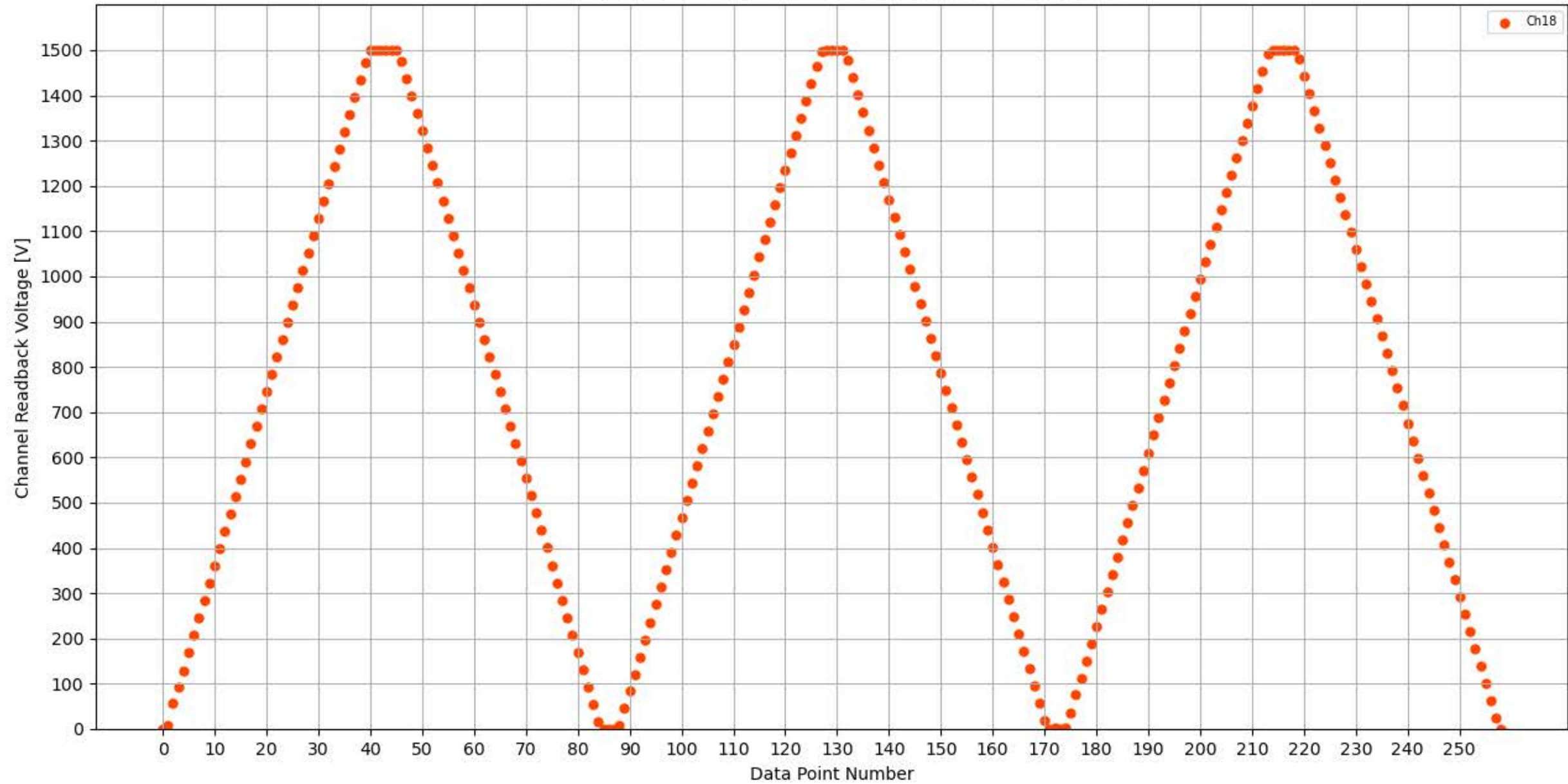
Voltage Ramp Test (Python) Bd #325, Slot #15, Ch #18
