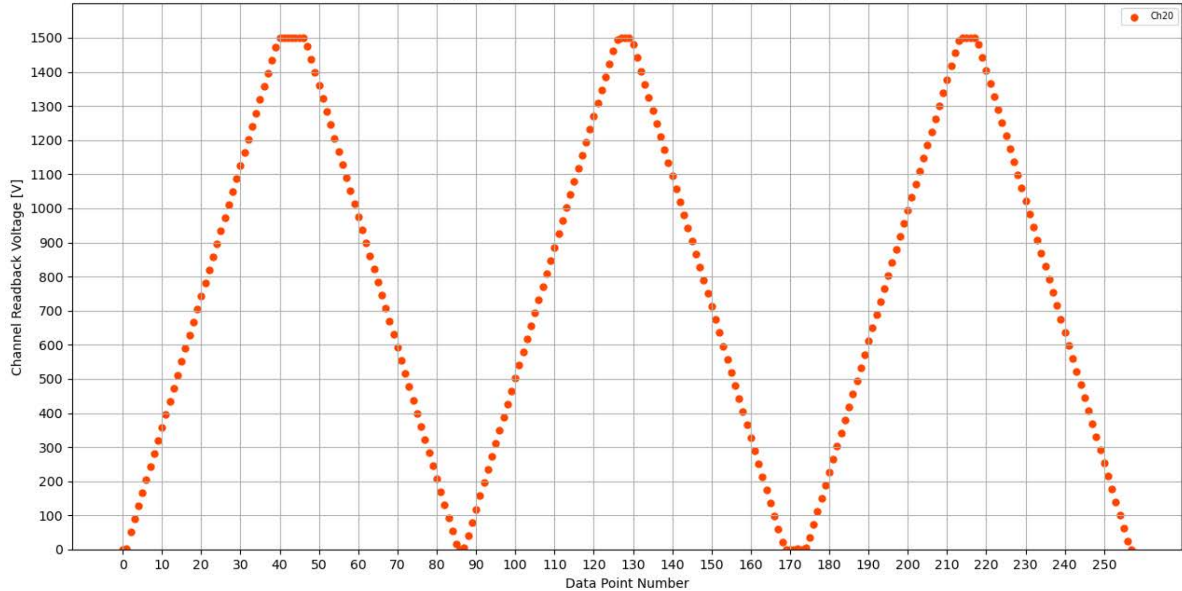
Voltage Ramp Test (Python) Bd #325, Slot #15, Ch #20
