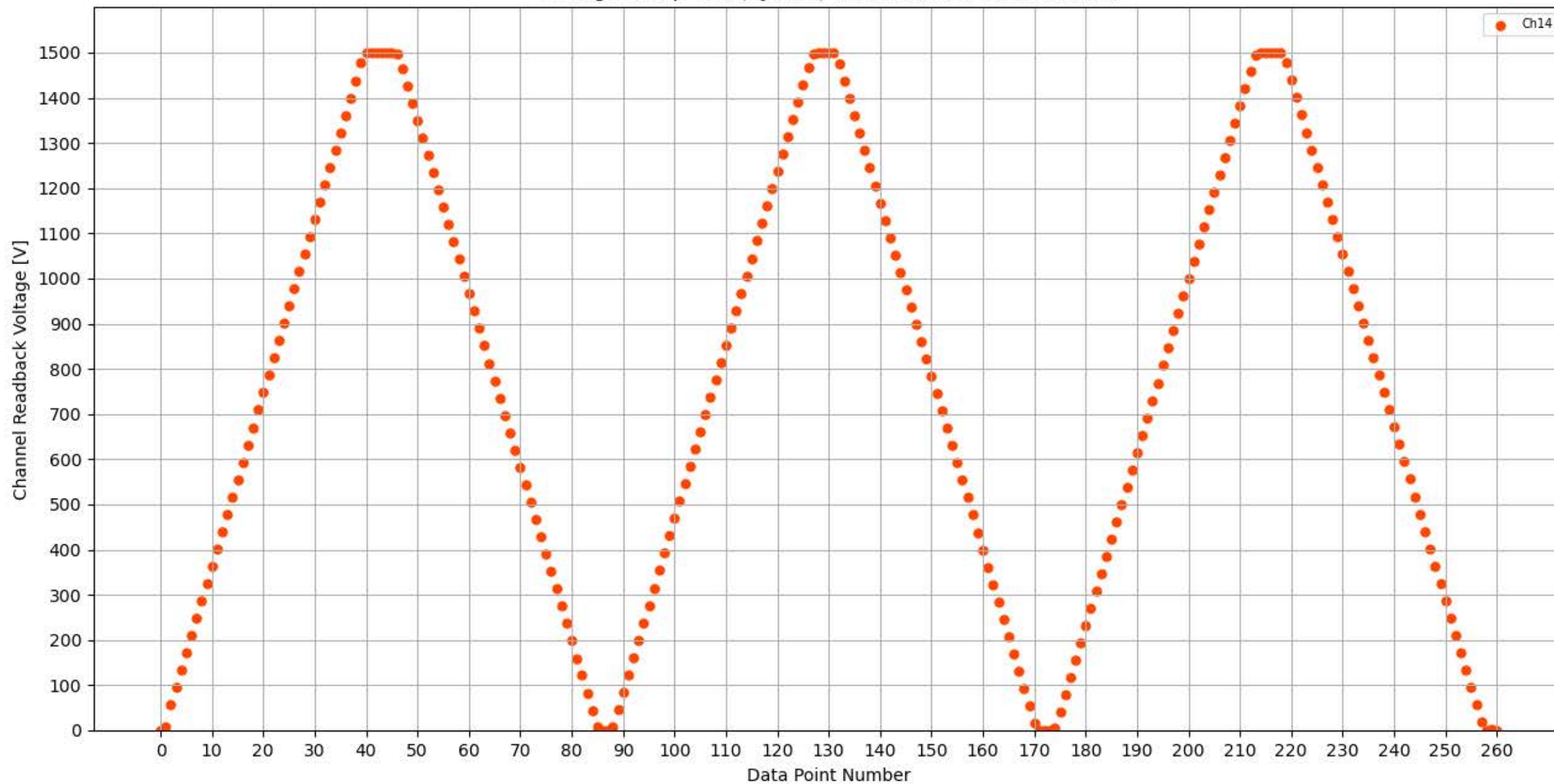
Voltage Ramp Test (Python) Bd #325, Slot #15, Ch #14
