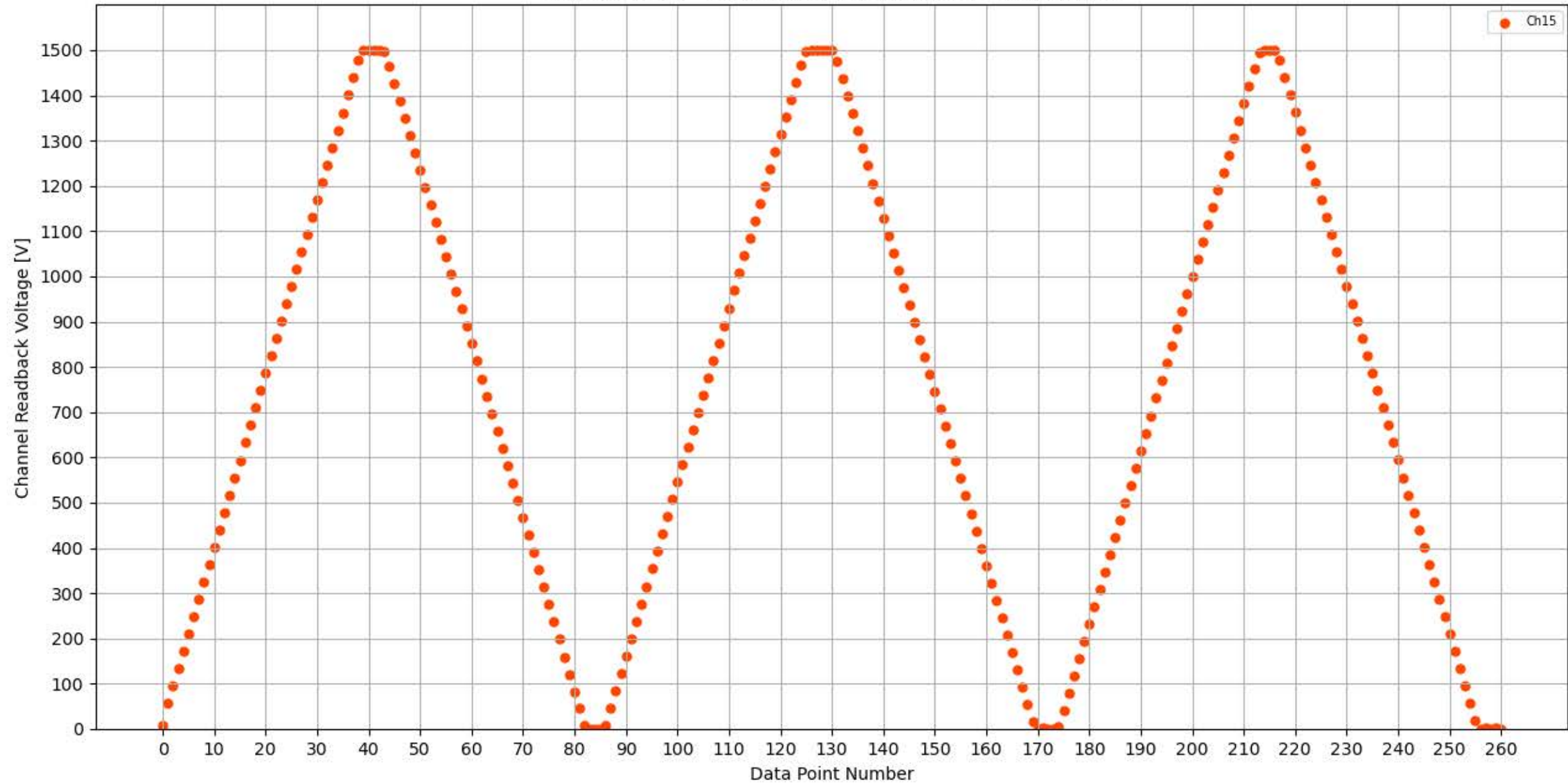
Voltage Ramp Test (Python) Bd #325, Slot #15, Ch #15
