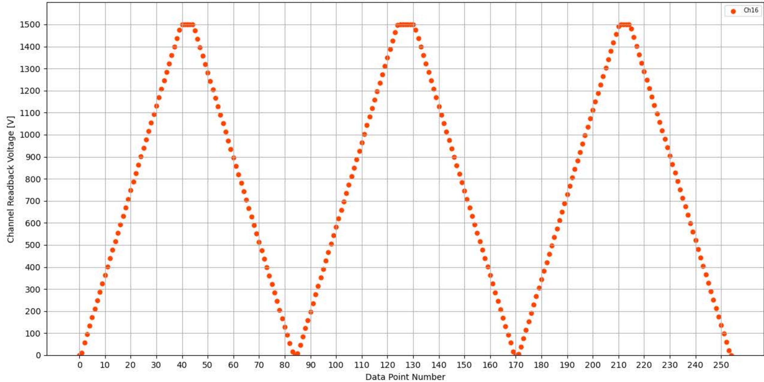
Voltage Ramp Test (Python) Bd #325, Slot #15, Ch #16
