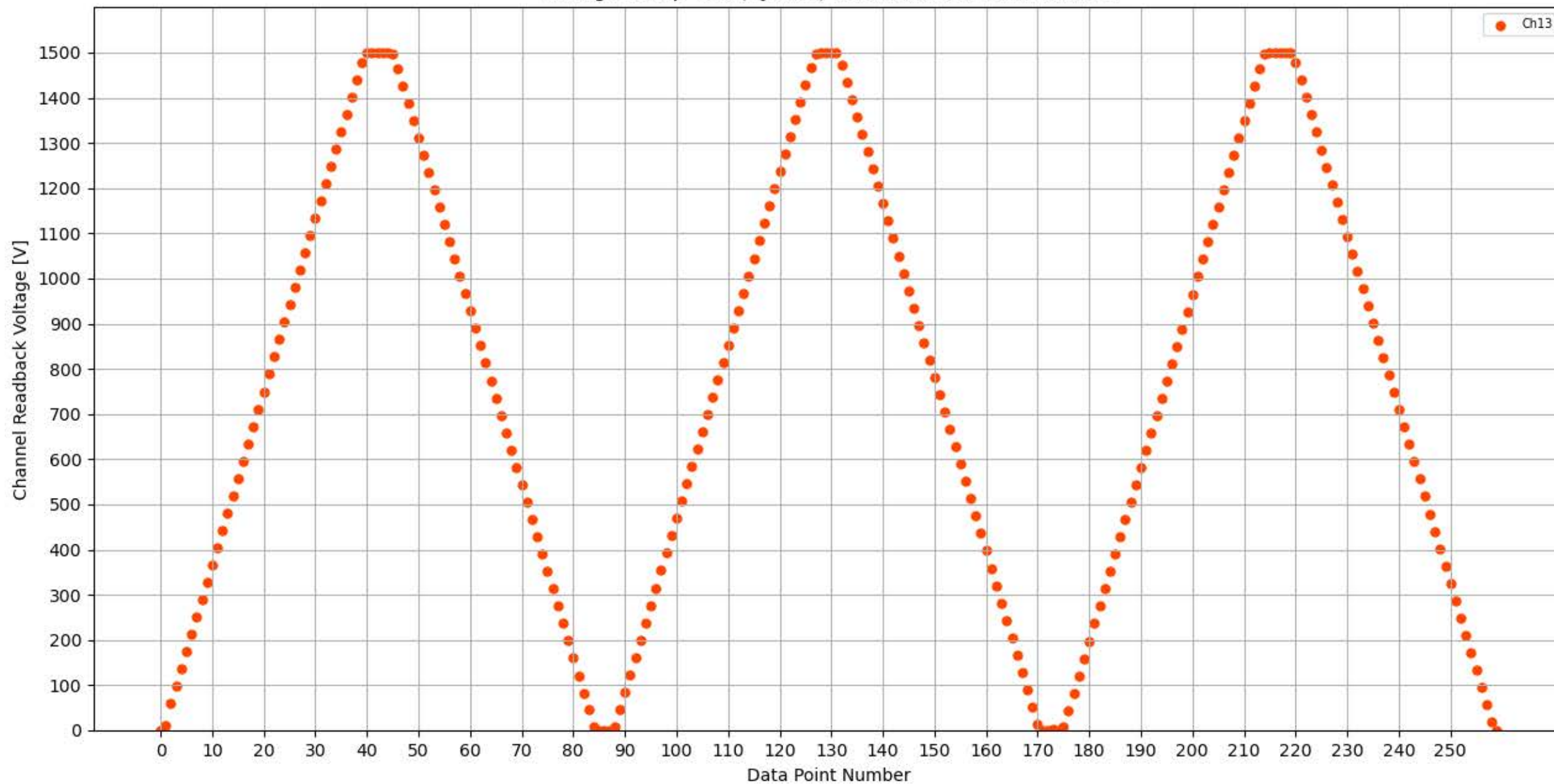
Voltage Ramp Test (Python) Bd #325, Slot #15, Ch #13
