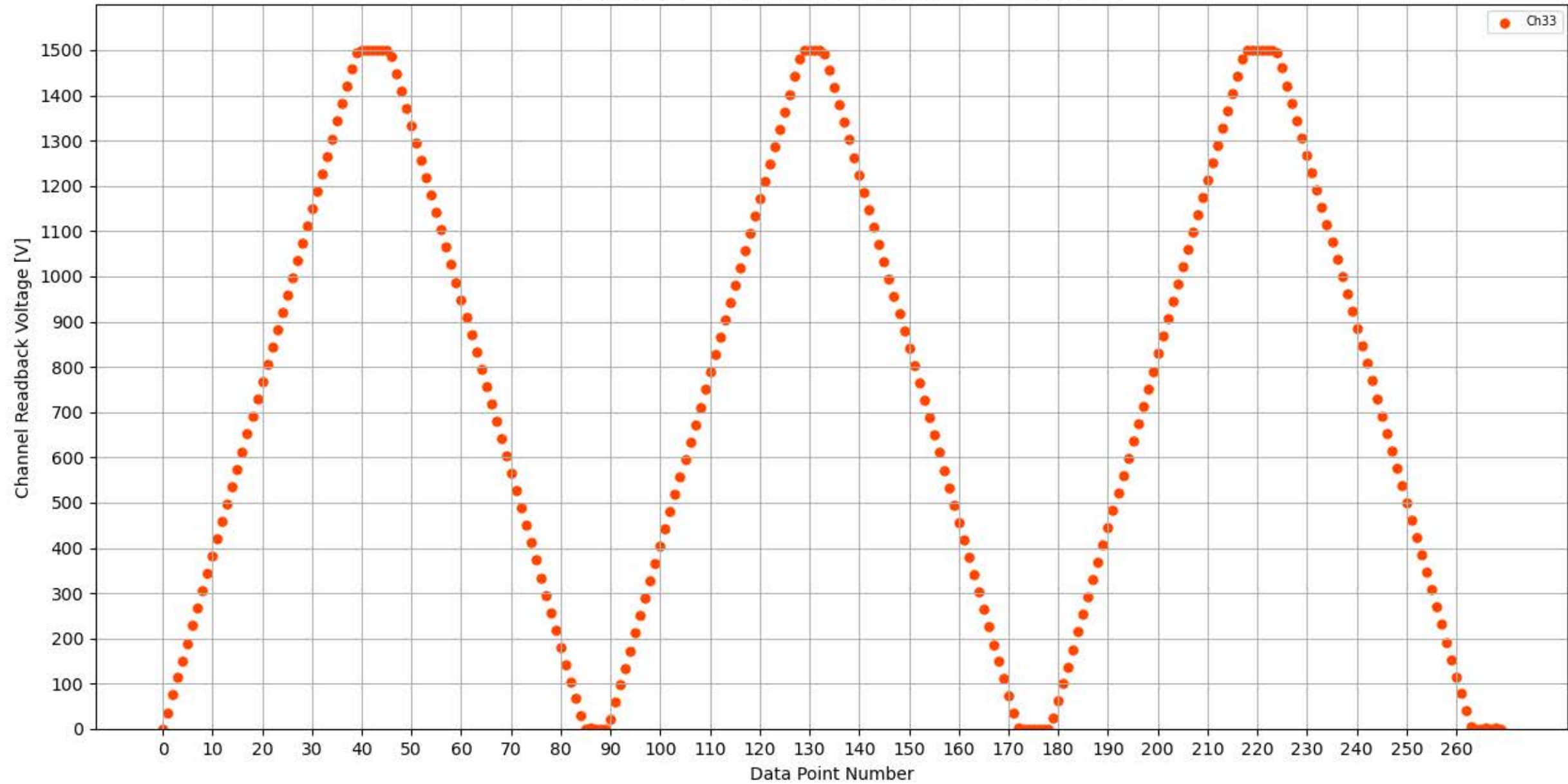
Voltage Ramp Test (Python) Bd #325, Slot #15, Ch #33
