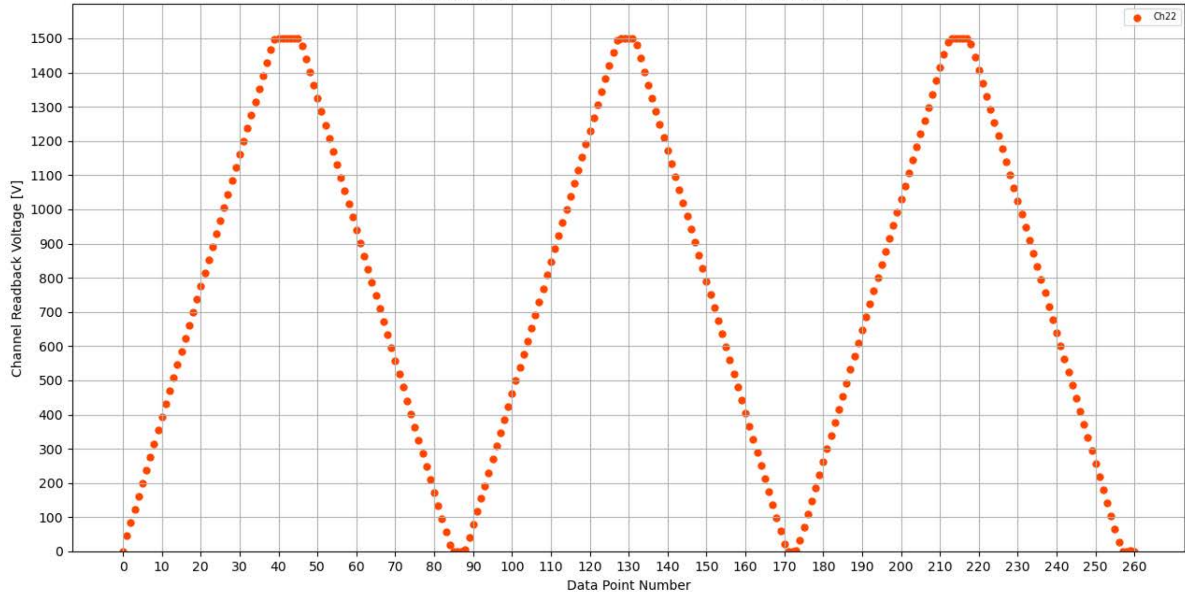
Voltage Ramp Test (Python) Bd #325, Slot #15, Ch #22
